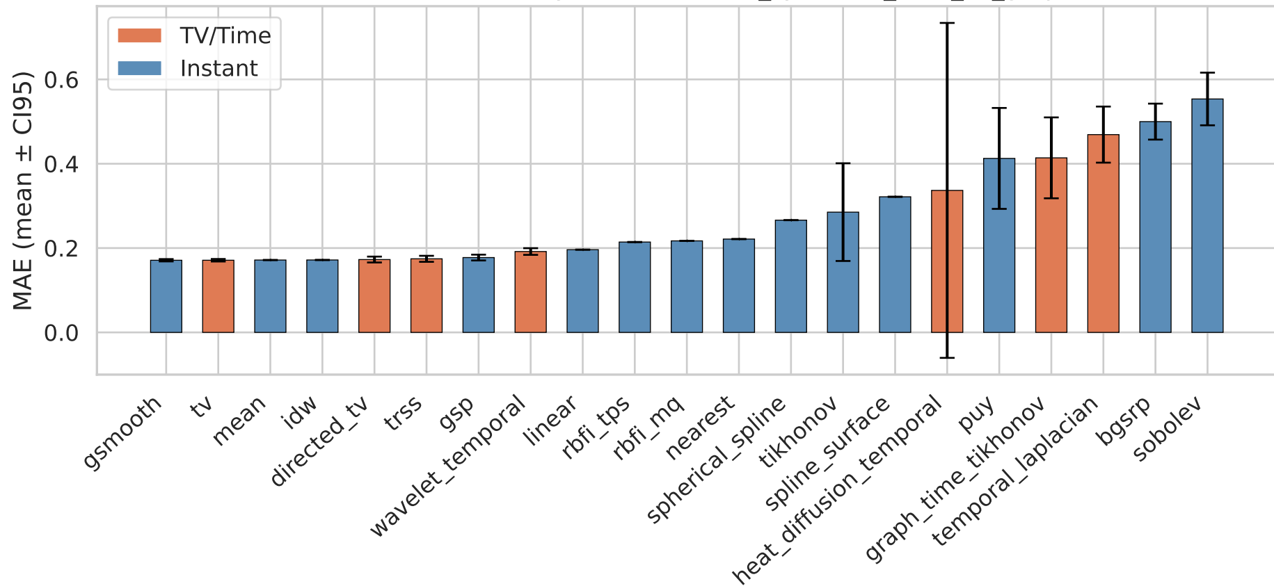
Mean Absolute Error by Method — it26_synthetic_beta_all_graphs
