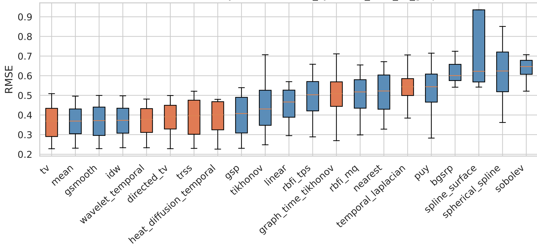
RMSE Distribution by Method — it26_synthetic_beta_all_graphs
