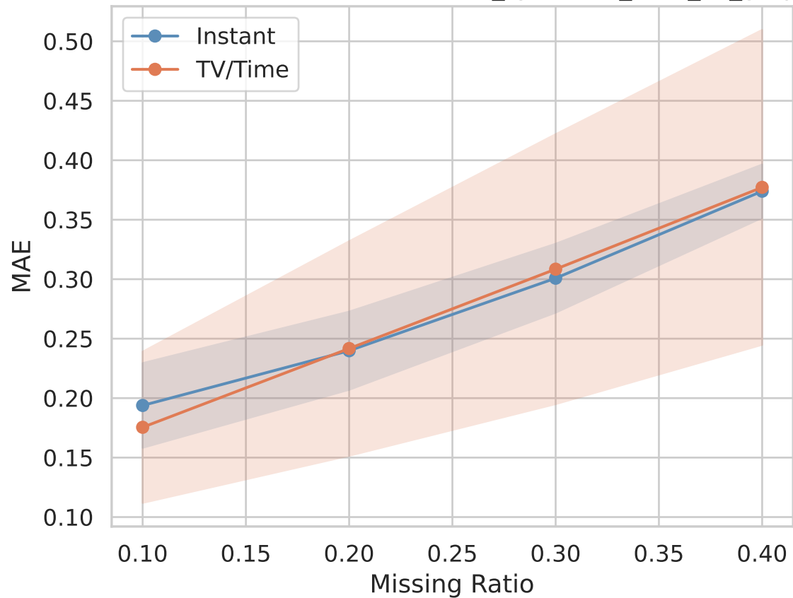
MAE — TV/Time vs Instant — it26_synthetic_beta_all_graphs
