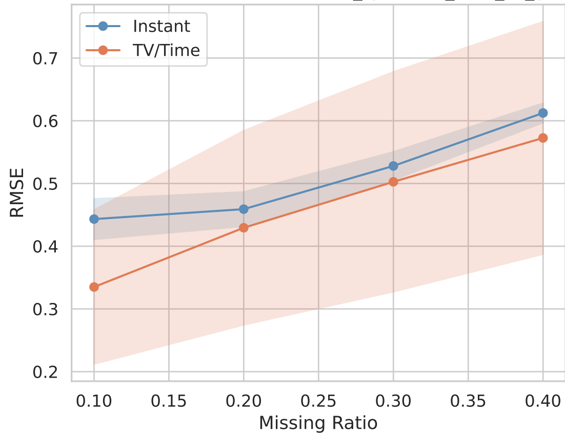
RMSE — TV/Time vs Instant — it26_synthetic_beta_all_graphs
