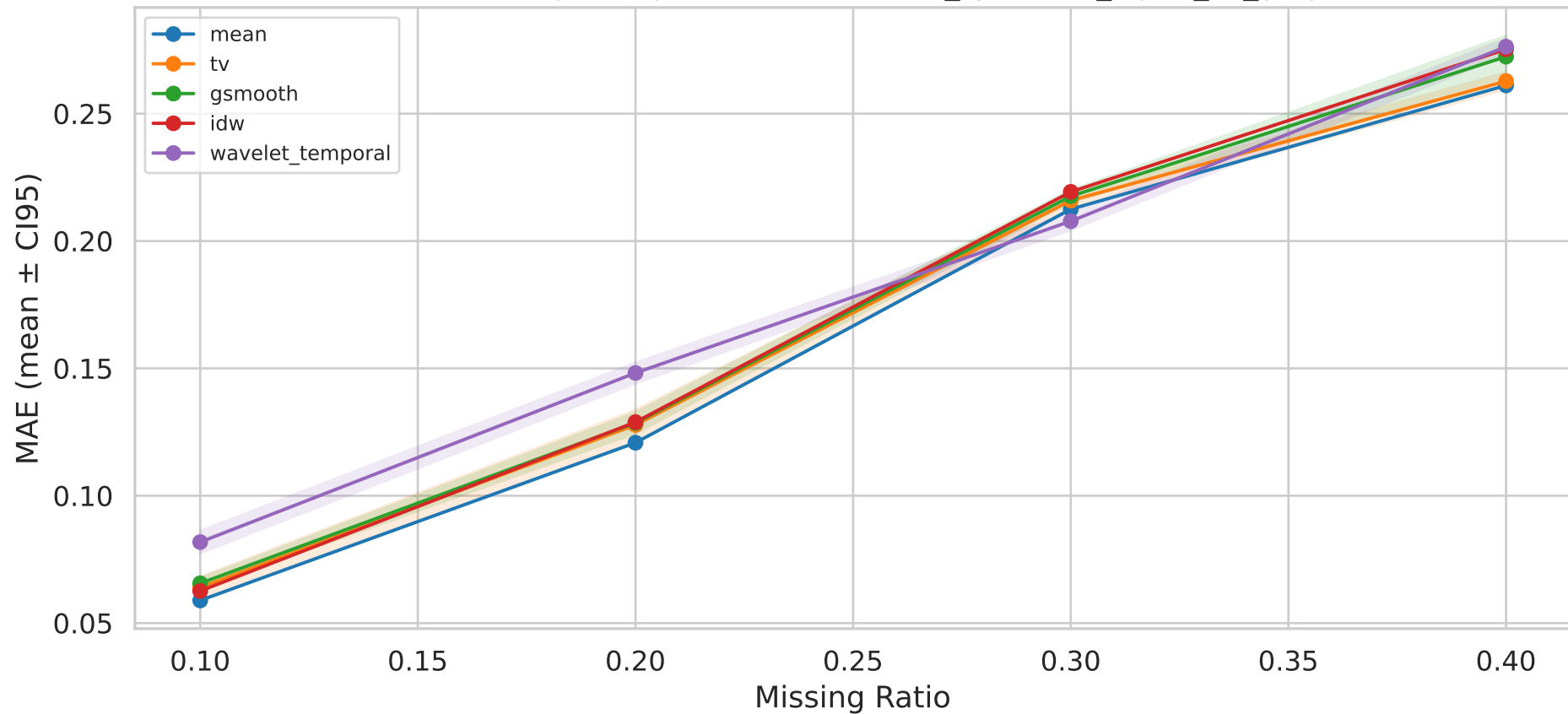
MAE Sensitivity — Top-5 Methods — it27_synthetic_alpha_all_graphs
