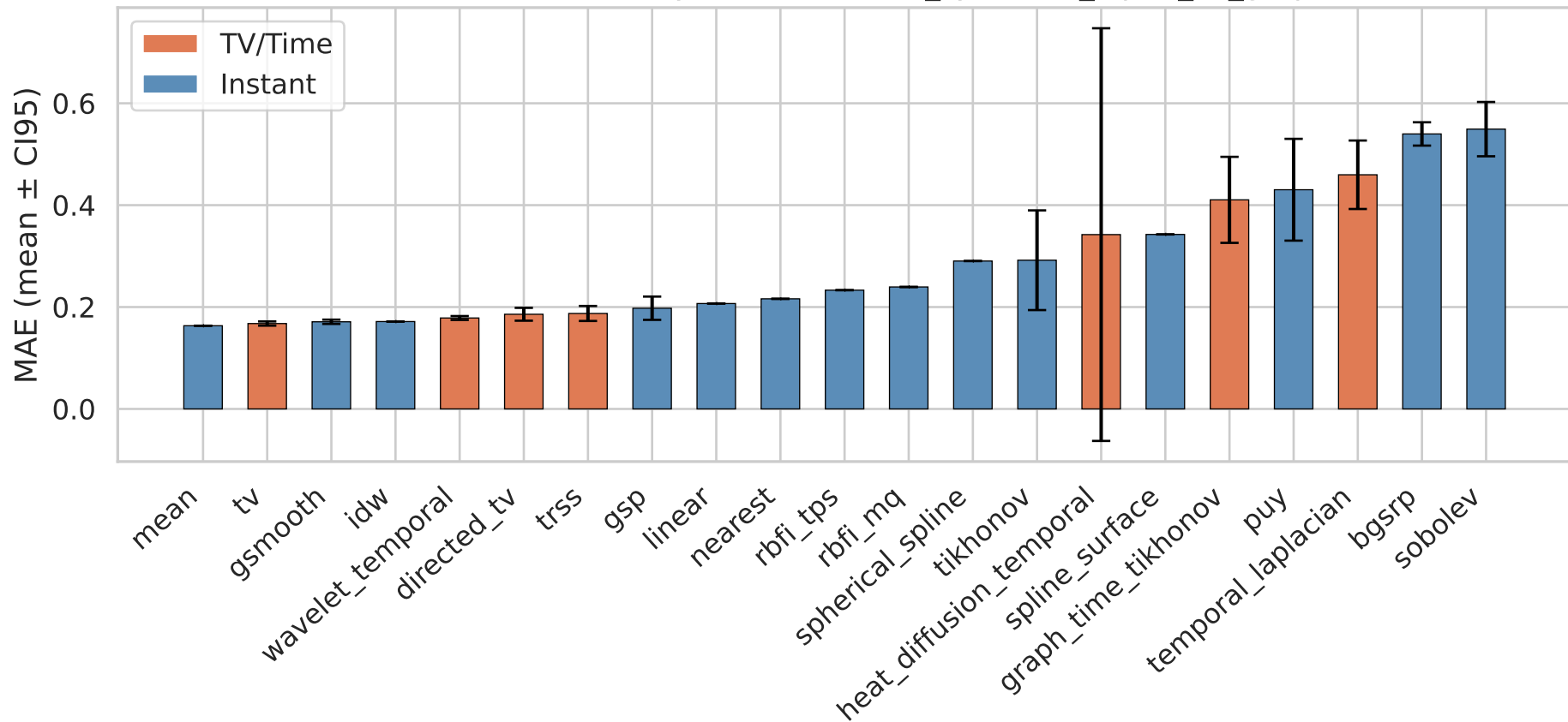
Mean Absolute Error by Method — it27_synthetic_alpha_all_graphs
