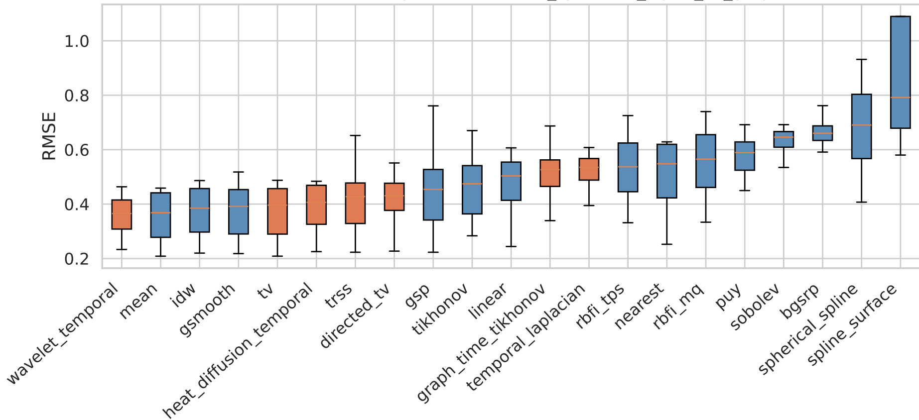
RMSE Distribution by Method — it27_synthetic_alpha_all_graphs
