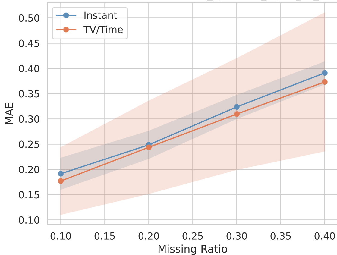
MAE — TV/Time vs Instant — it27_synthetic_alpha_all_graphs
