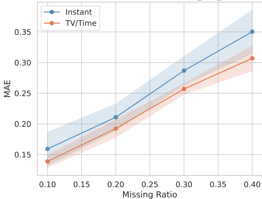
MAE — TV/Time vs Instant — it28_nnk_3syn
