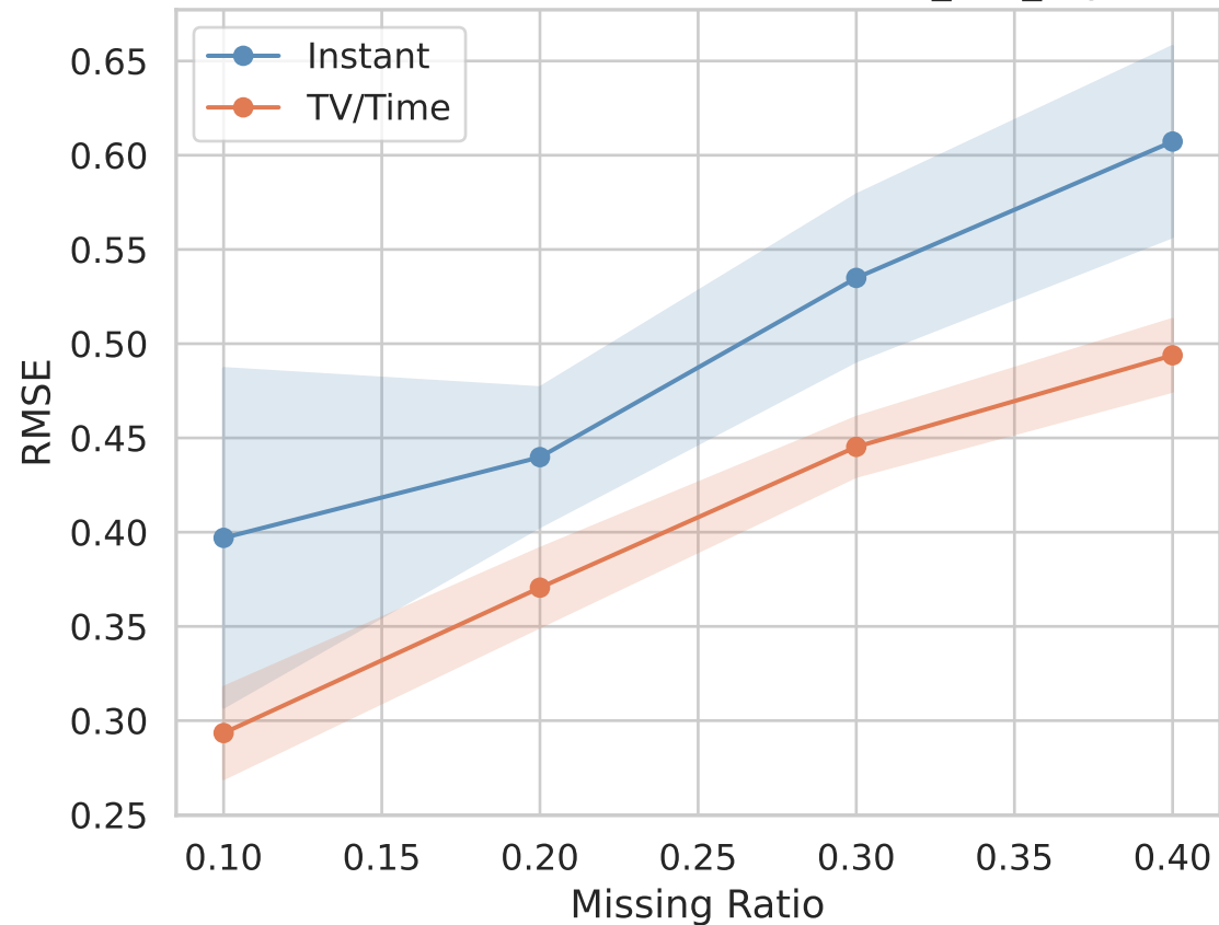
RMSE — TV/Time vs Instant — it28_nnk_3syn
