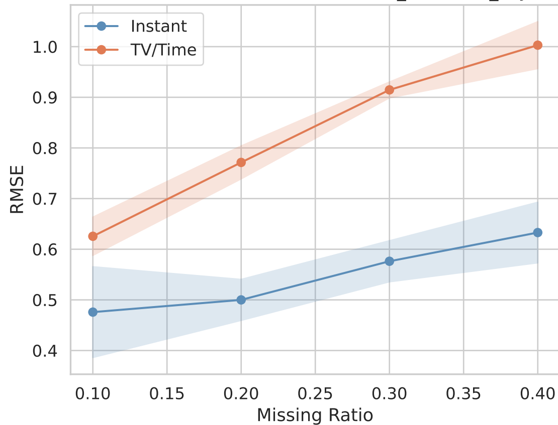
RMSE — TV/Time vs Instant — it29_kalofolias_3syn
