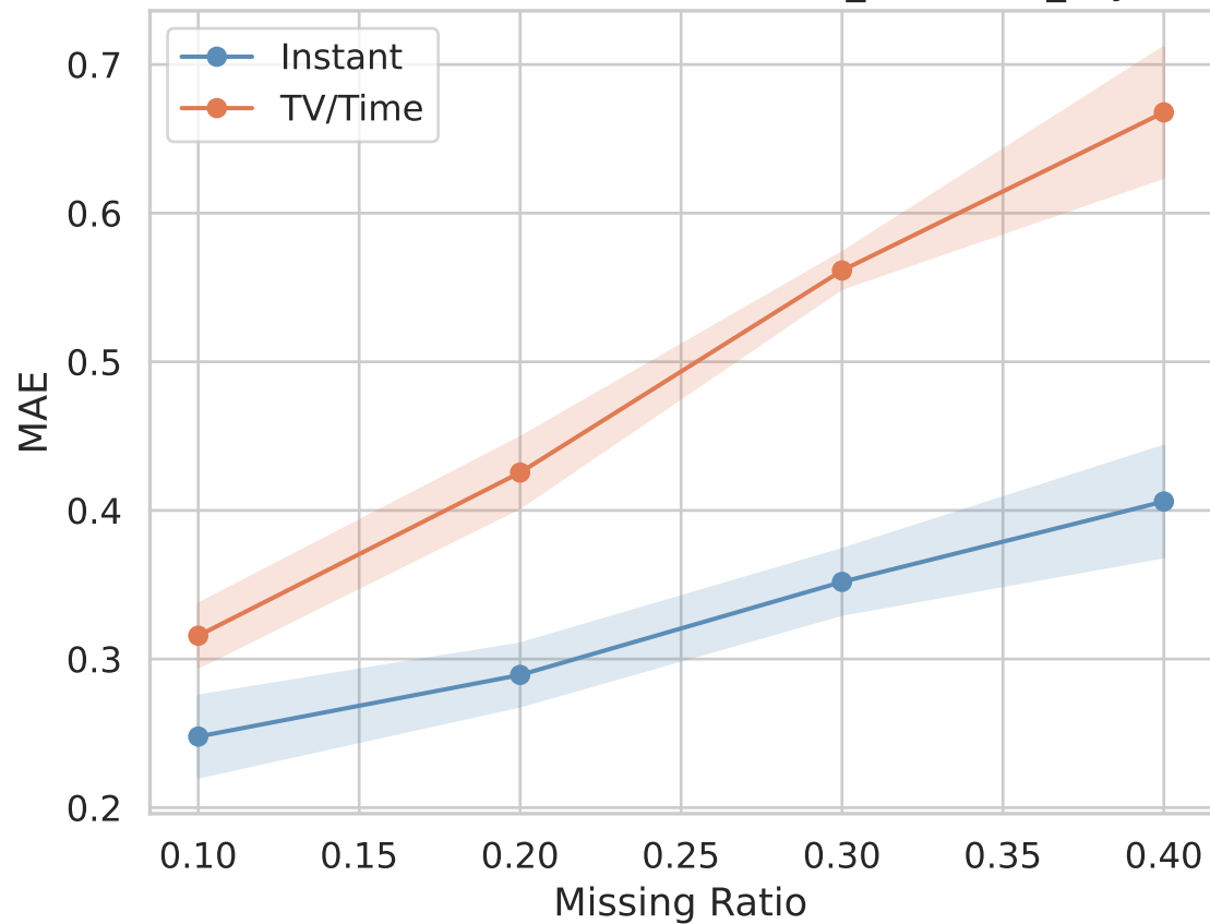
MAE — TV/Time vs Instant — it29_kalofolias_3syn
