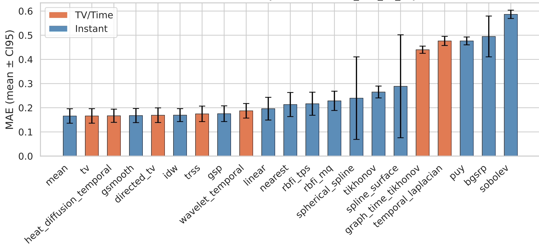
Mean Absolute Error by Method — it30_knn_k5_3syn
