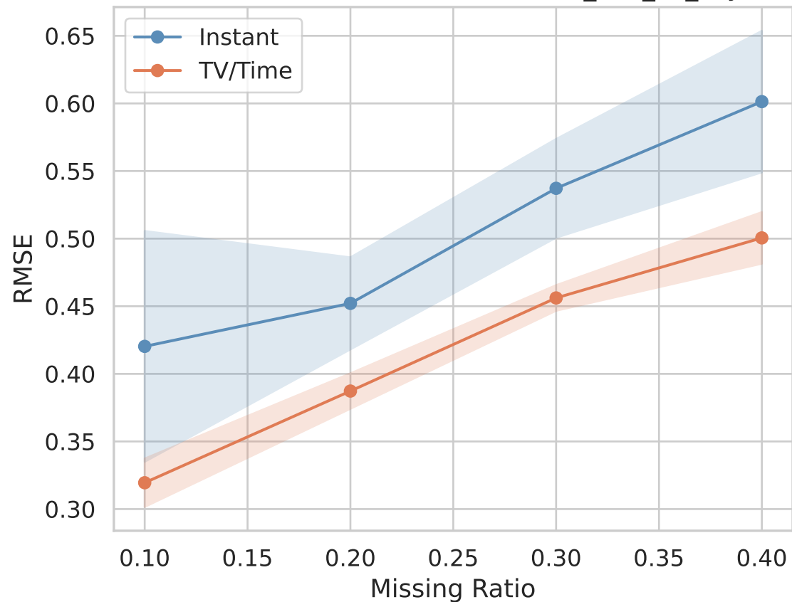
RMSE — TV/Time vs Instant — it30_knn_k5_3syn
