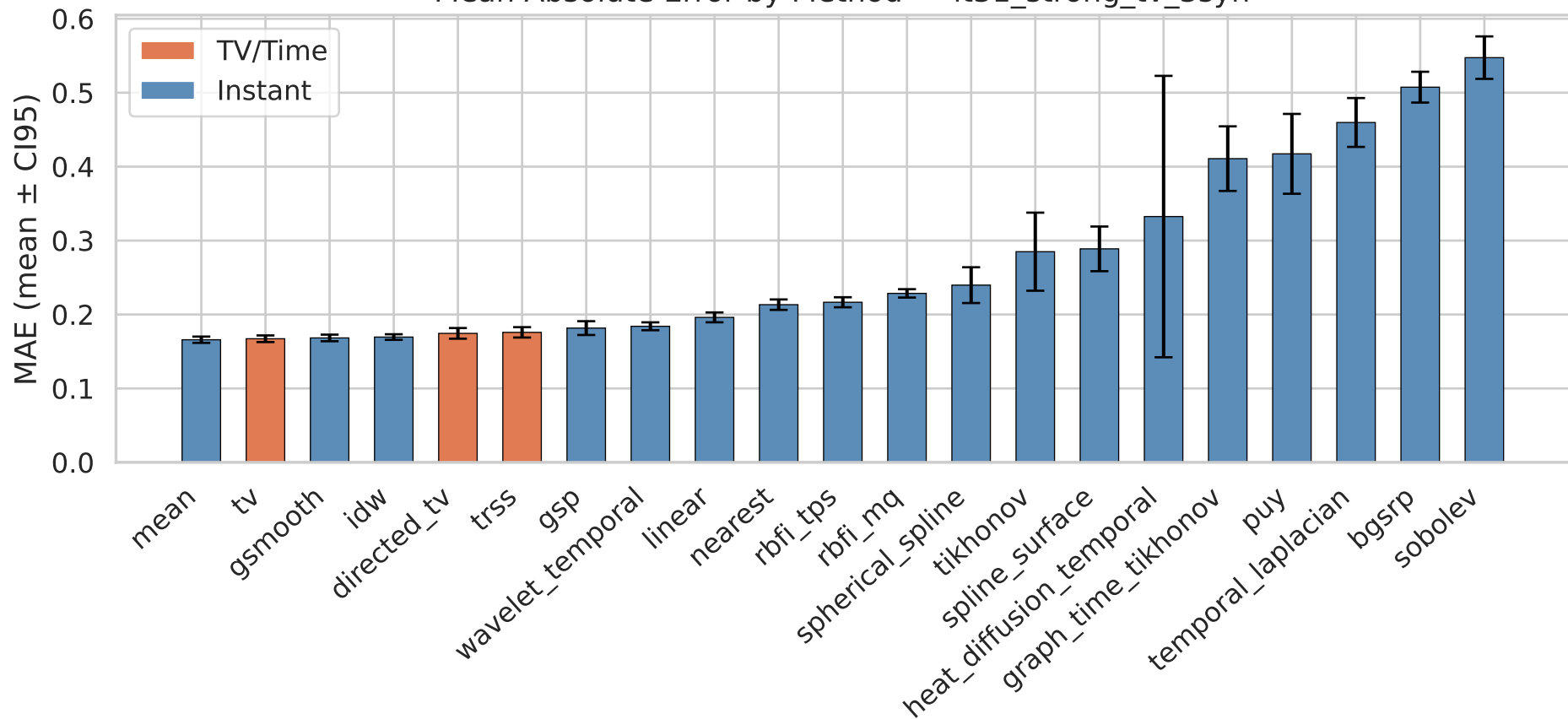
Mean Absolute Error by Method — it31_strong_tv_3syn
