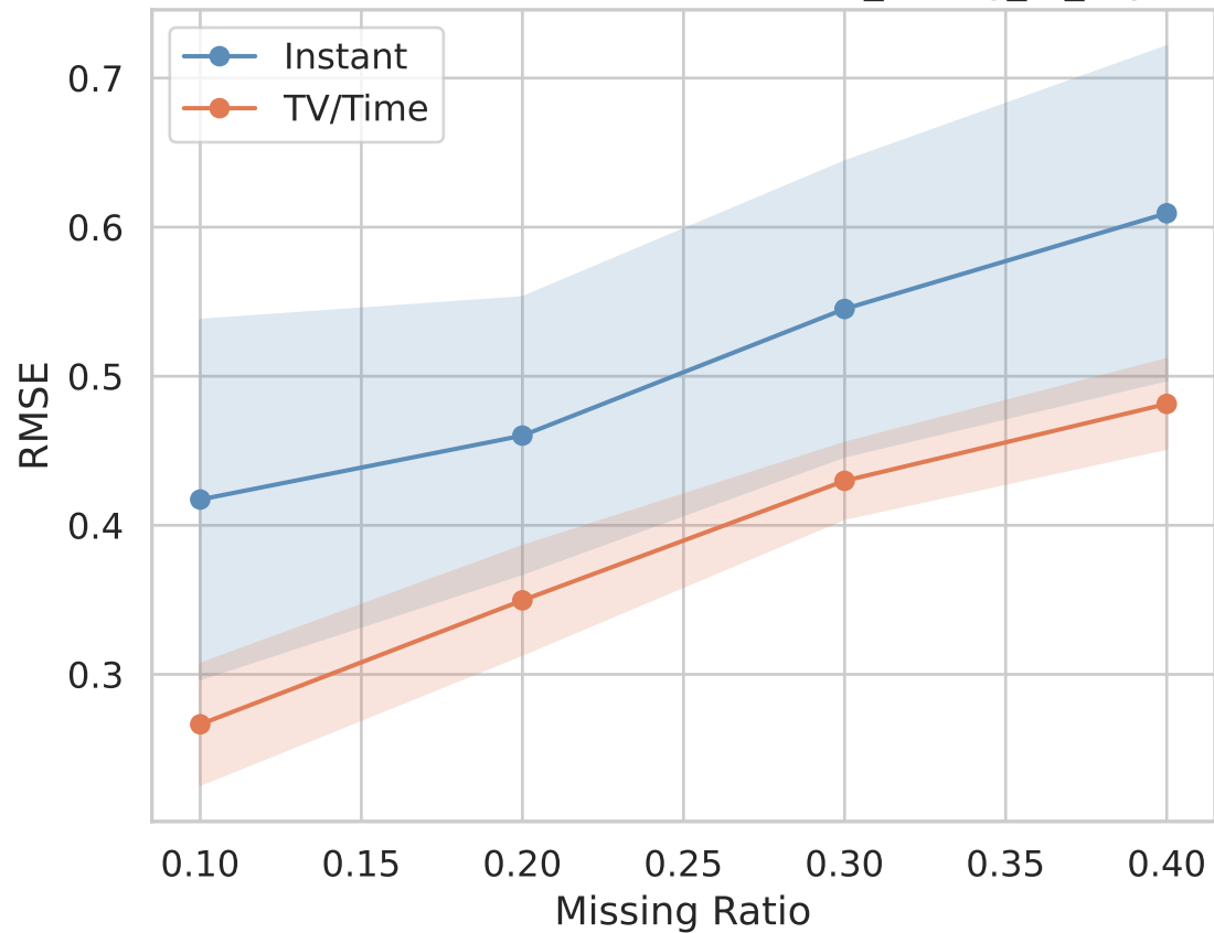
RMSE — TV/Time vs Instant — it31_strong_tv_3syn
