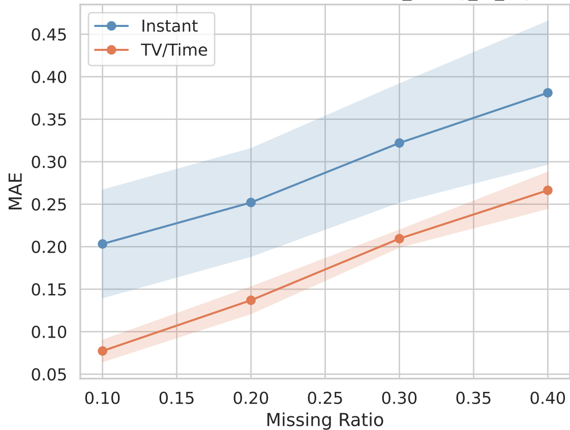
MAE — TV/Time vs Instant — it31_strong_tv_3syn
