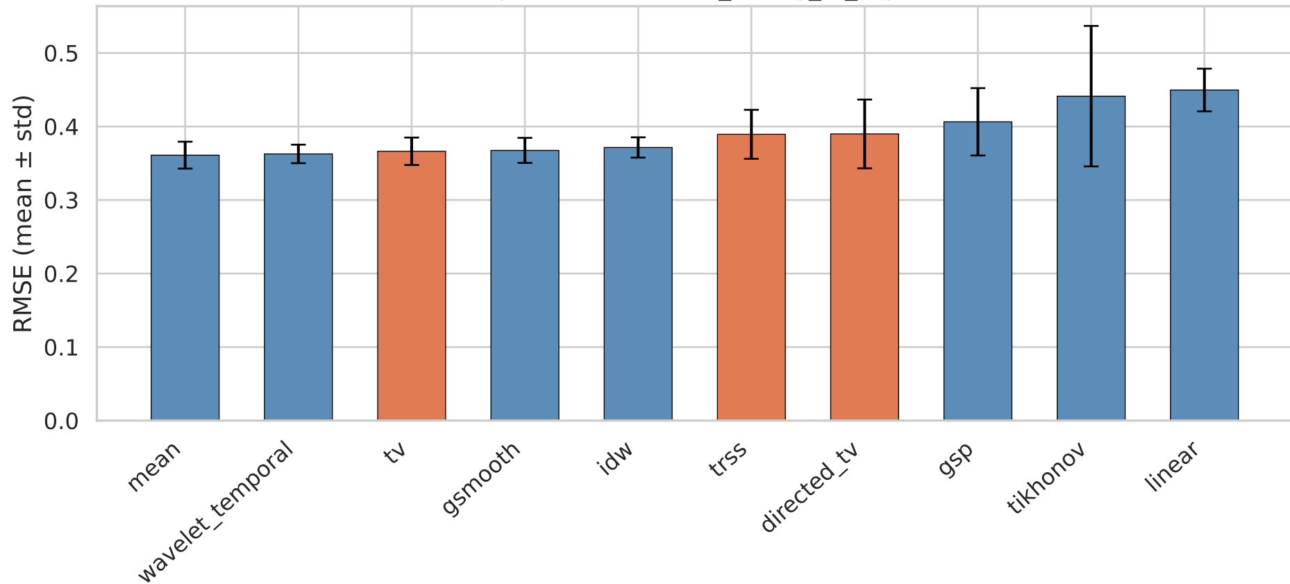
Top-10 RMSE — it31_strong_tv_3syn
