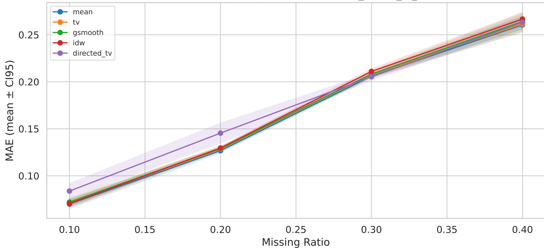
MAE Sensitivity — Top-5 Methods — it31_strong_tv_3syn
