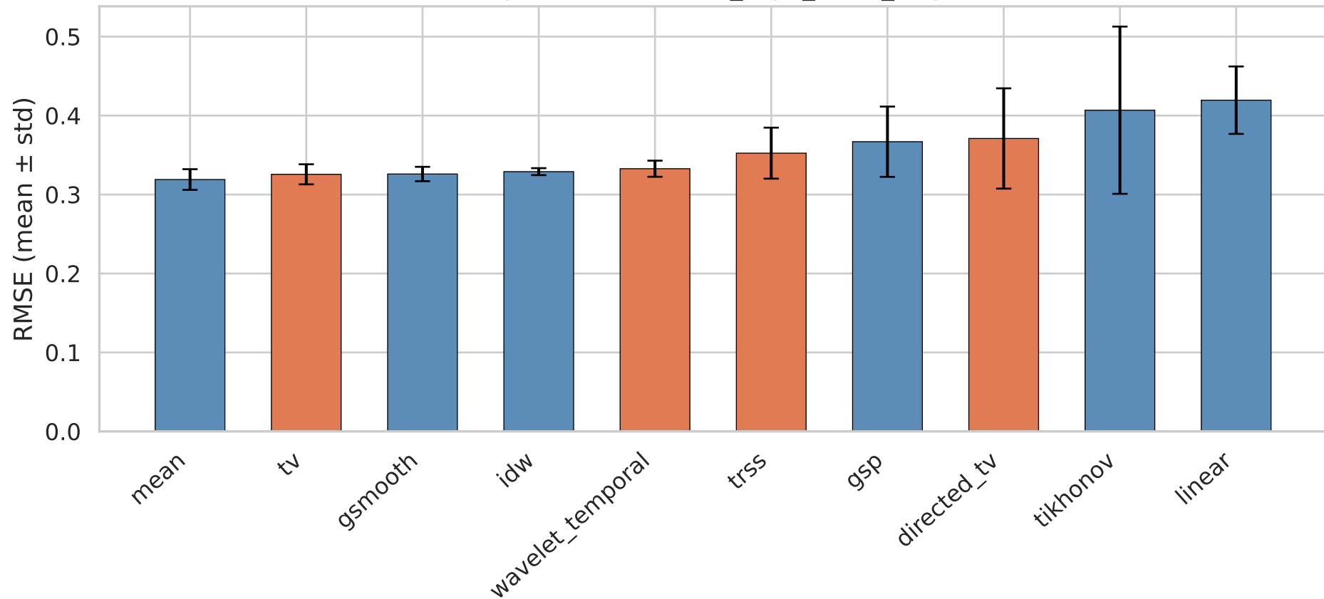
Top-10 RMSE — it32_3syn_mr20_only
