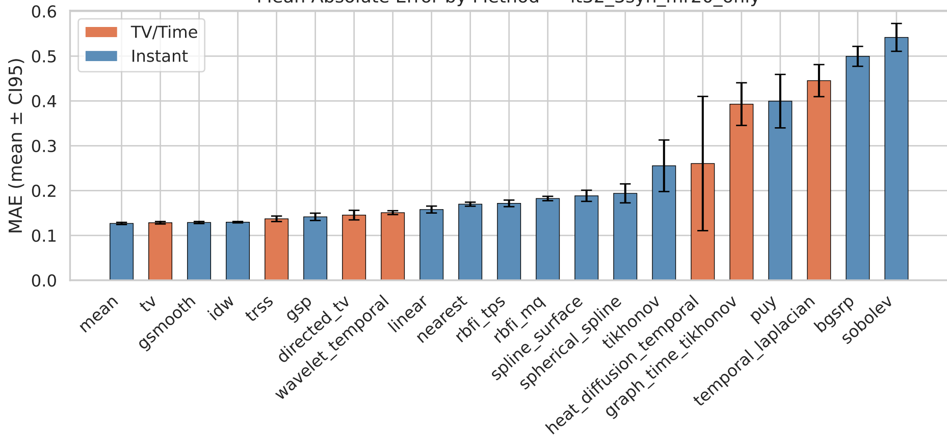
Mean Absolute Error by Method — it32_3syn_mr20_only
