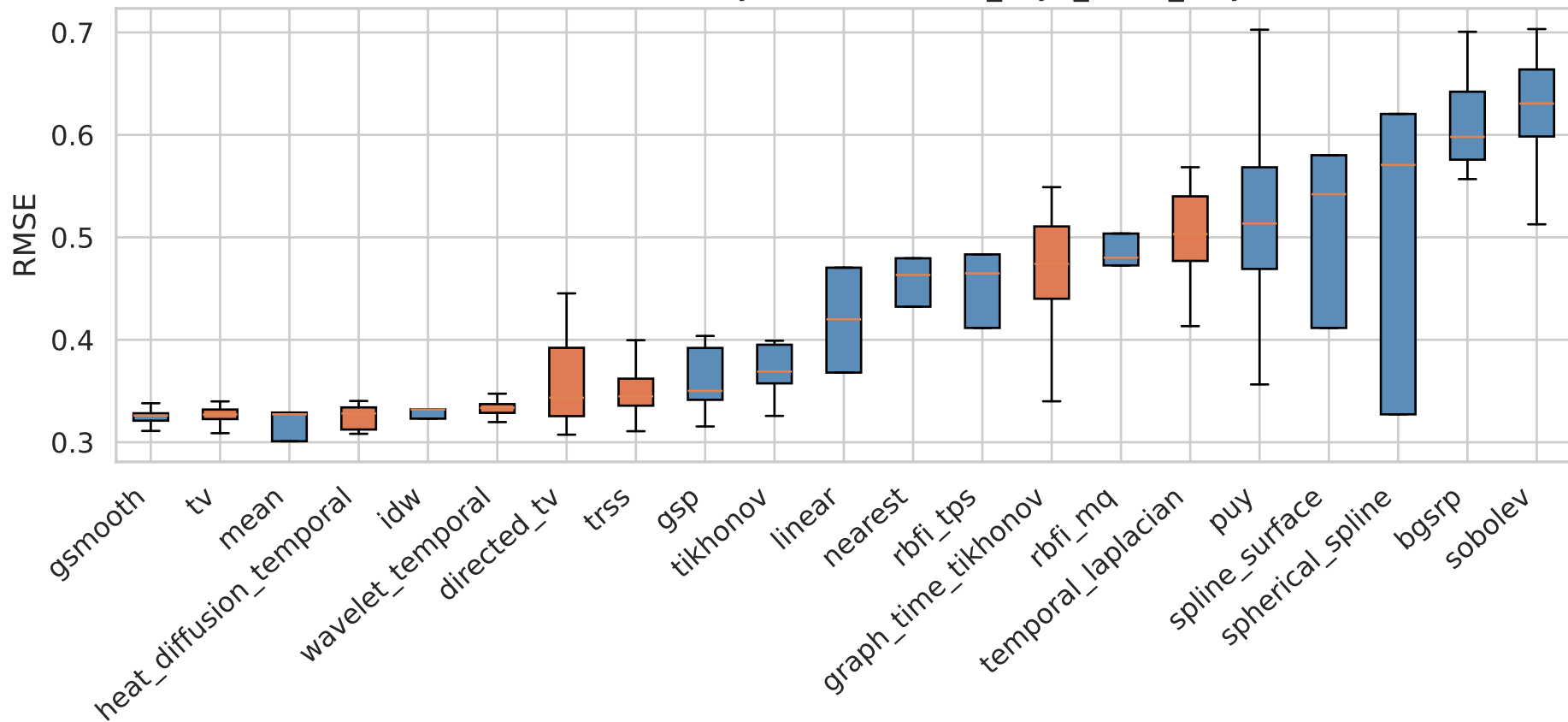
RMSE Distribution by Method — it32_3syn_mr20_only
