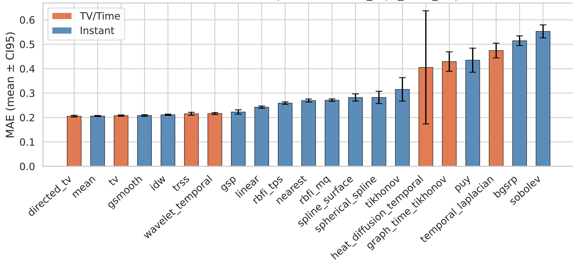
Mean Absolute Error by Method — it33_3syn_mr30_only
