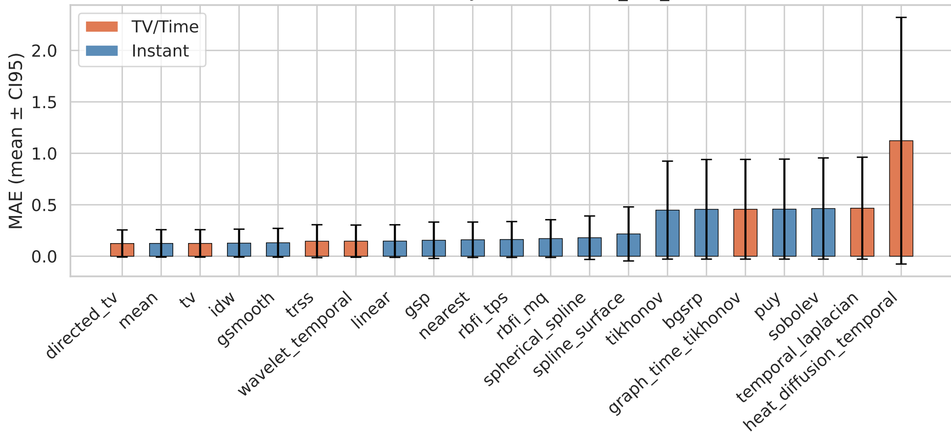
Mean Absolute Error by Method — it35_all4_kalofolias
