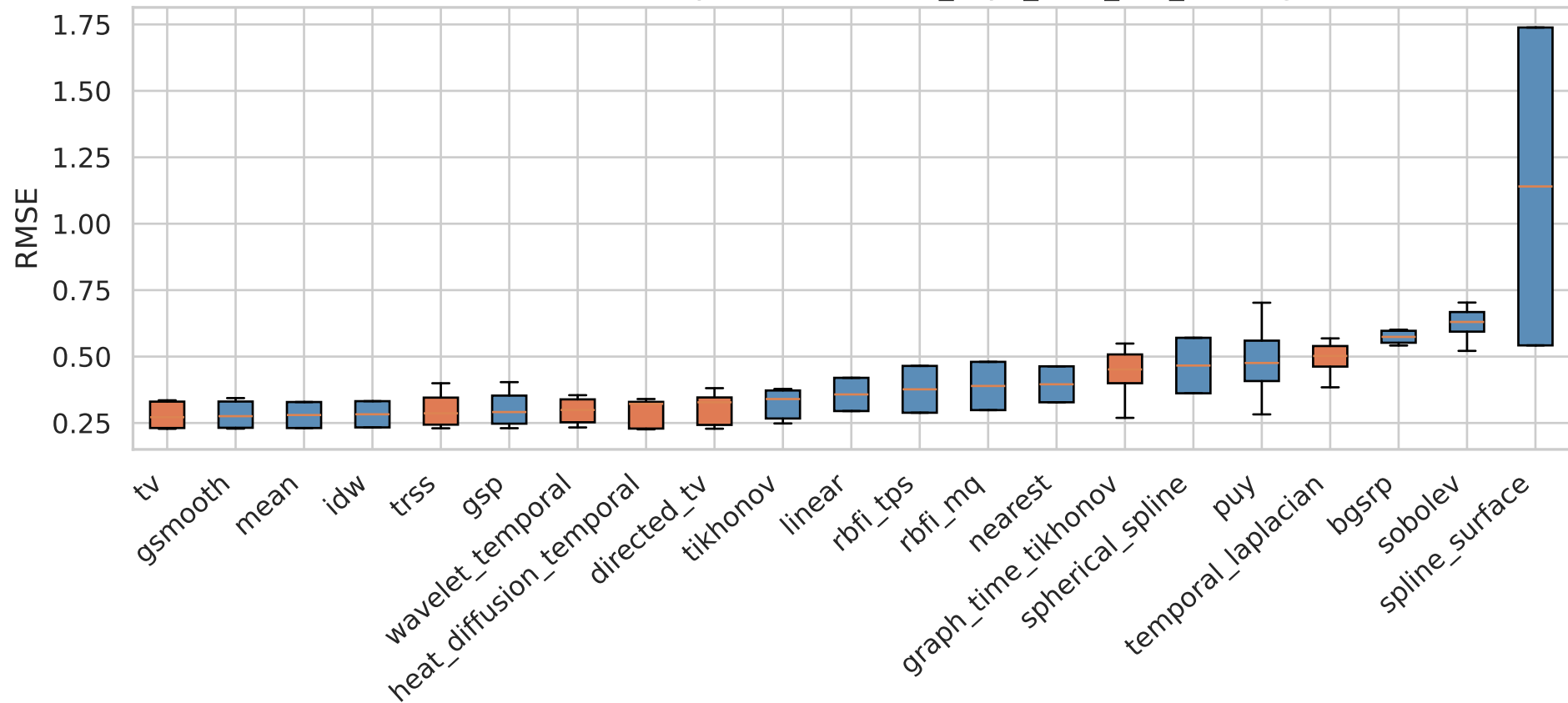
RMSE Distribution by Method — it36_3syn_beta_low_missing
