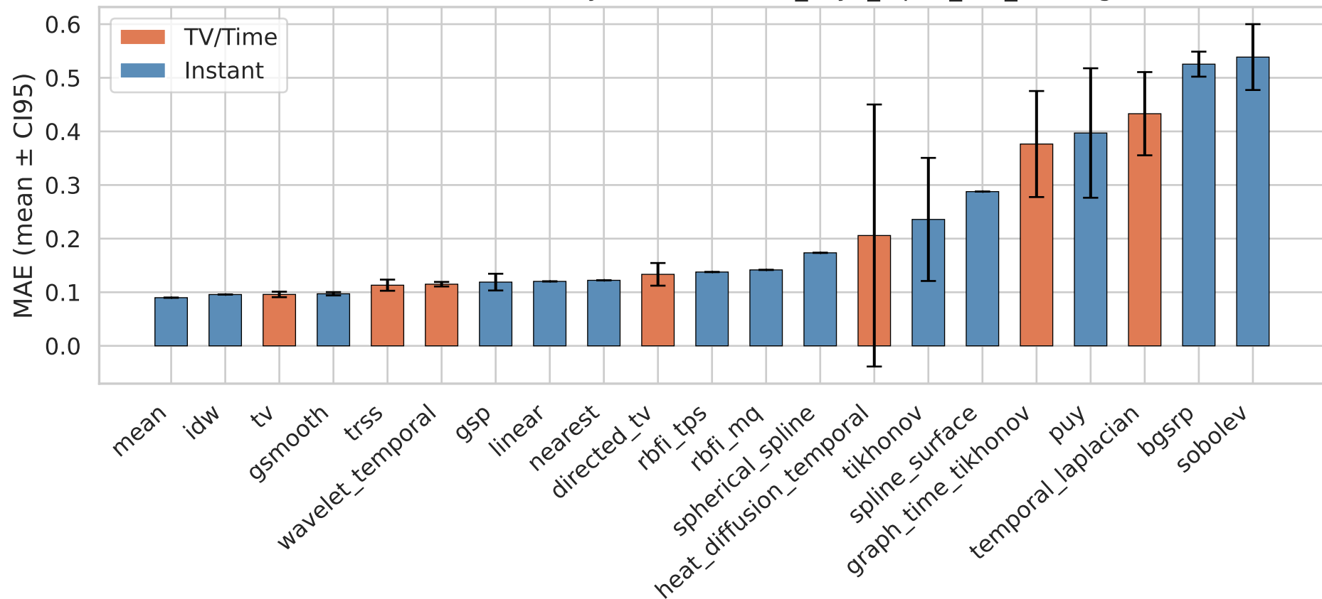
Mean Absolute Error by Method — it37_3syn_alpha_low_missing
