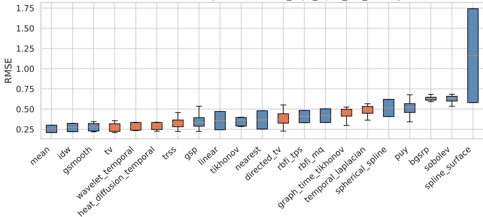
RMSE Distribution by Method — it37_3syn_alpha_low_missing
