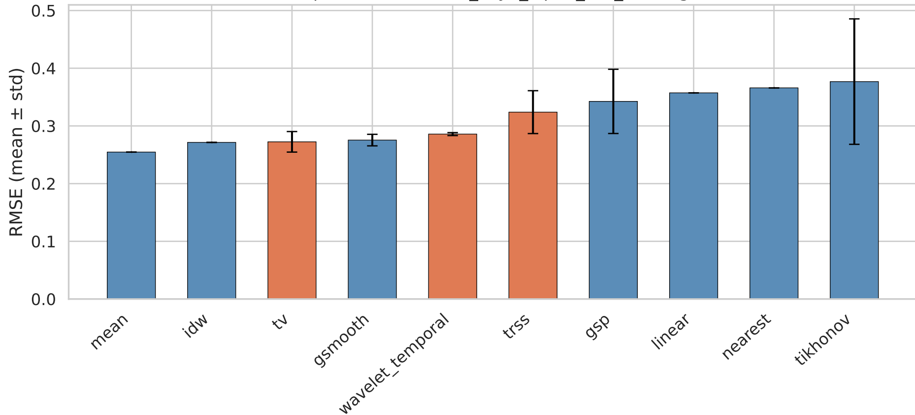
Top-10 RMSE — it37_3syn_alpha_low_missing
