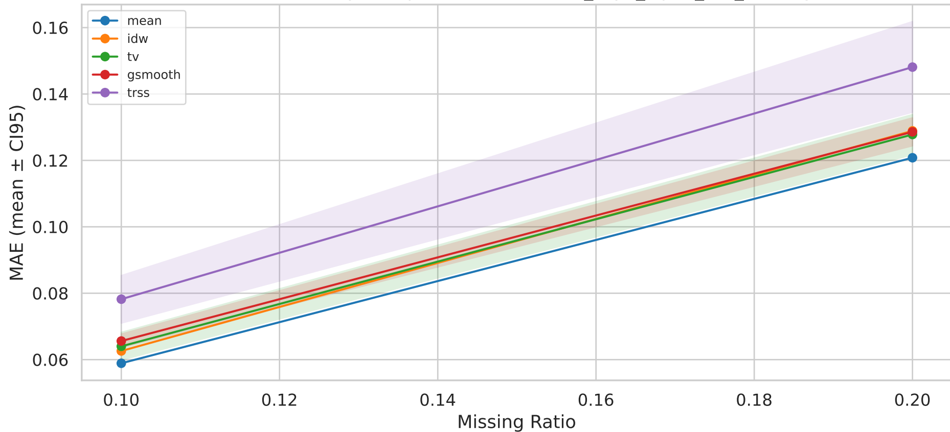
MAE Sensitivity — Top-5 Methods — it37_3syn_alpha_low_missing
