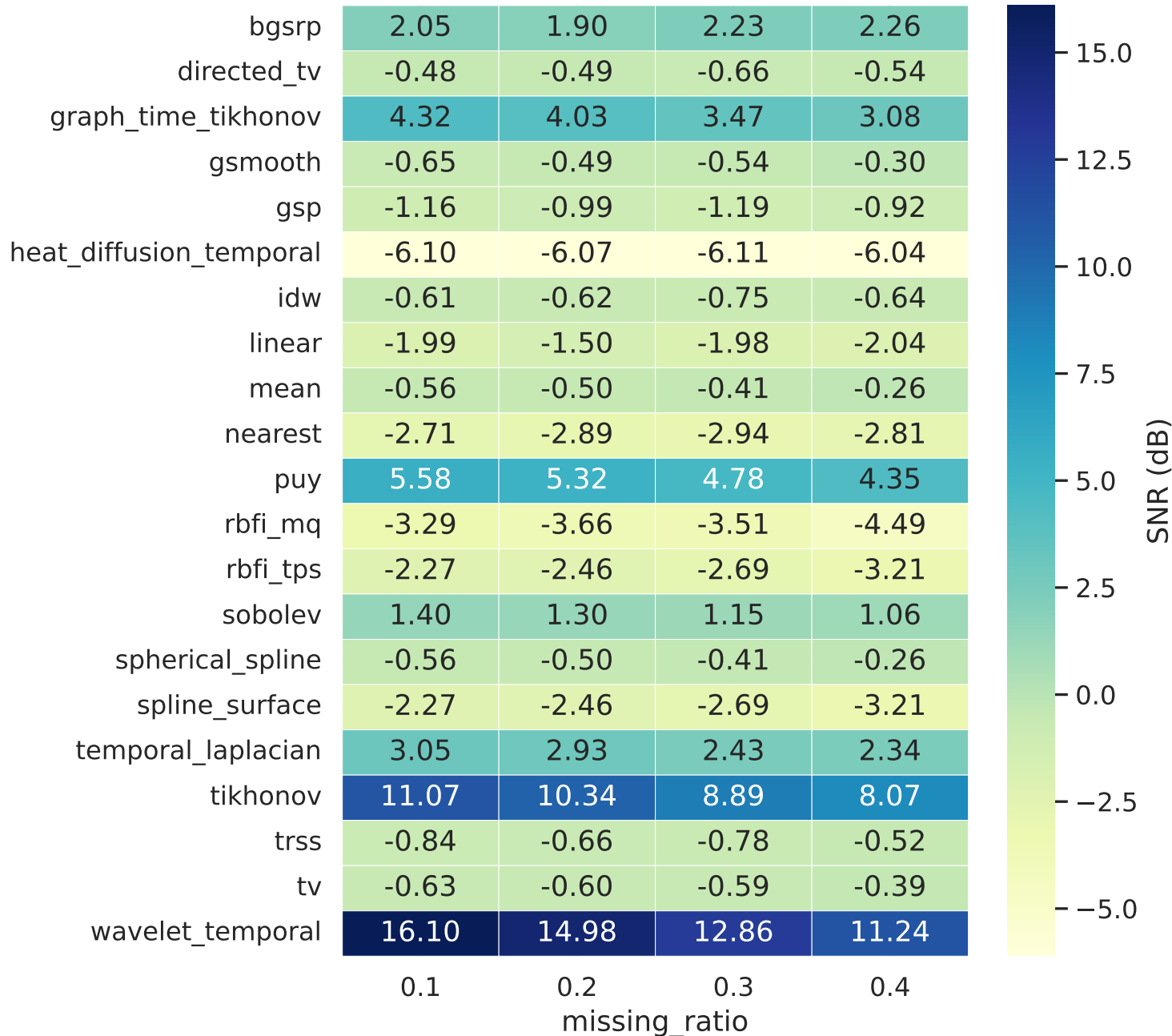
Mean SNR — Method × Scenario — it38_broad_gaussian_kalofolias_nnk
