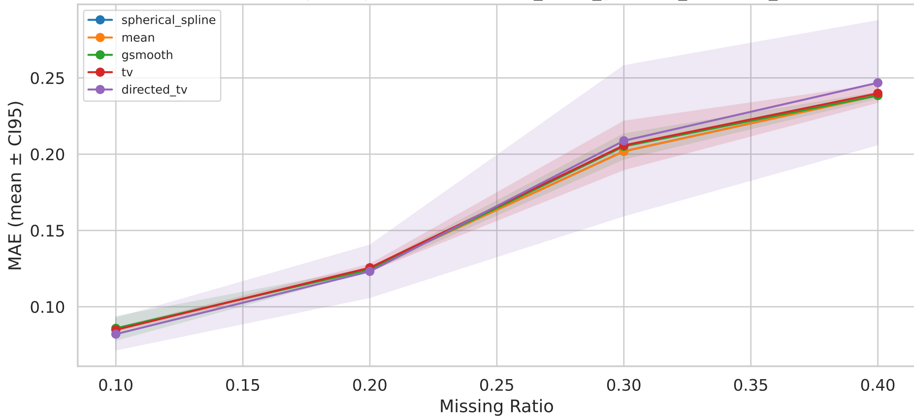
MAE Sensitivity — Top-5 Methods — it38_broad_gaussian_kalofolias_nnk
