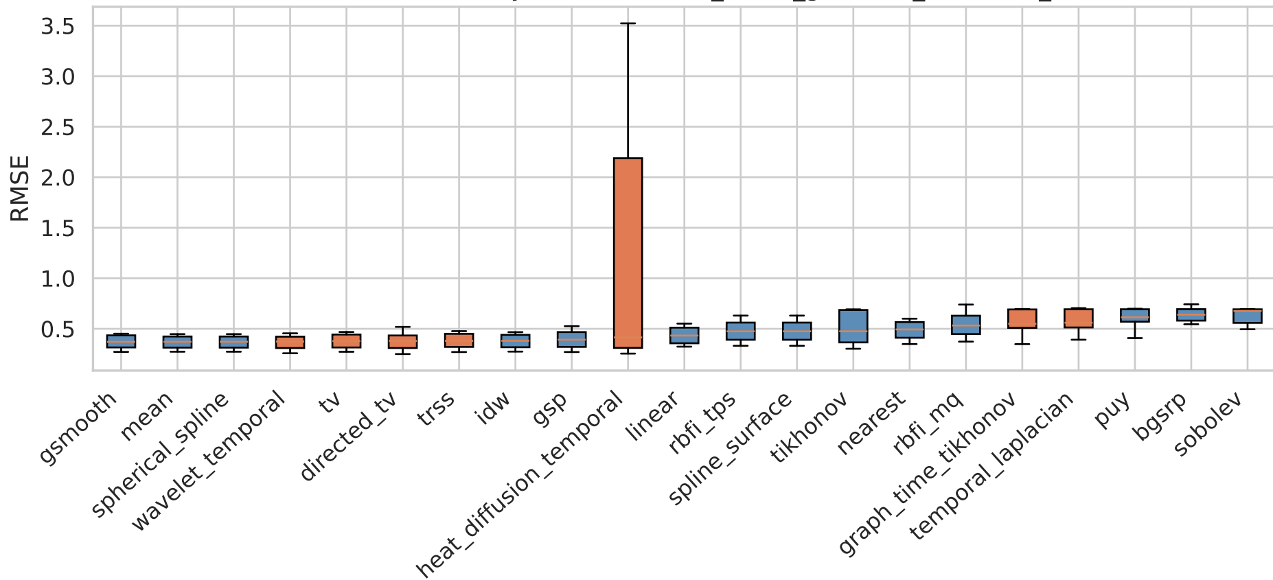
RMSE Distribution by Method — it38_broad_gaussian_kalofolias_nnk
