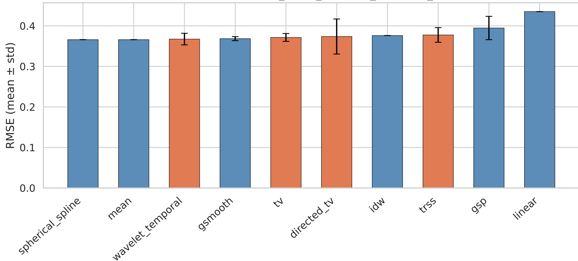
Top-10 RMSE — it38_broad_gaussian_kalofolias_nnk
