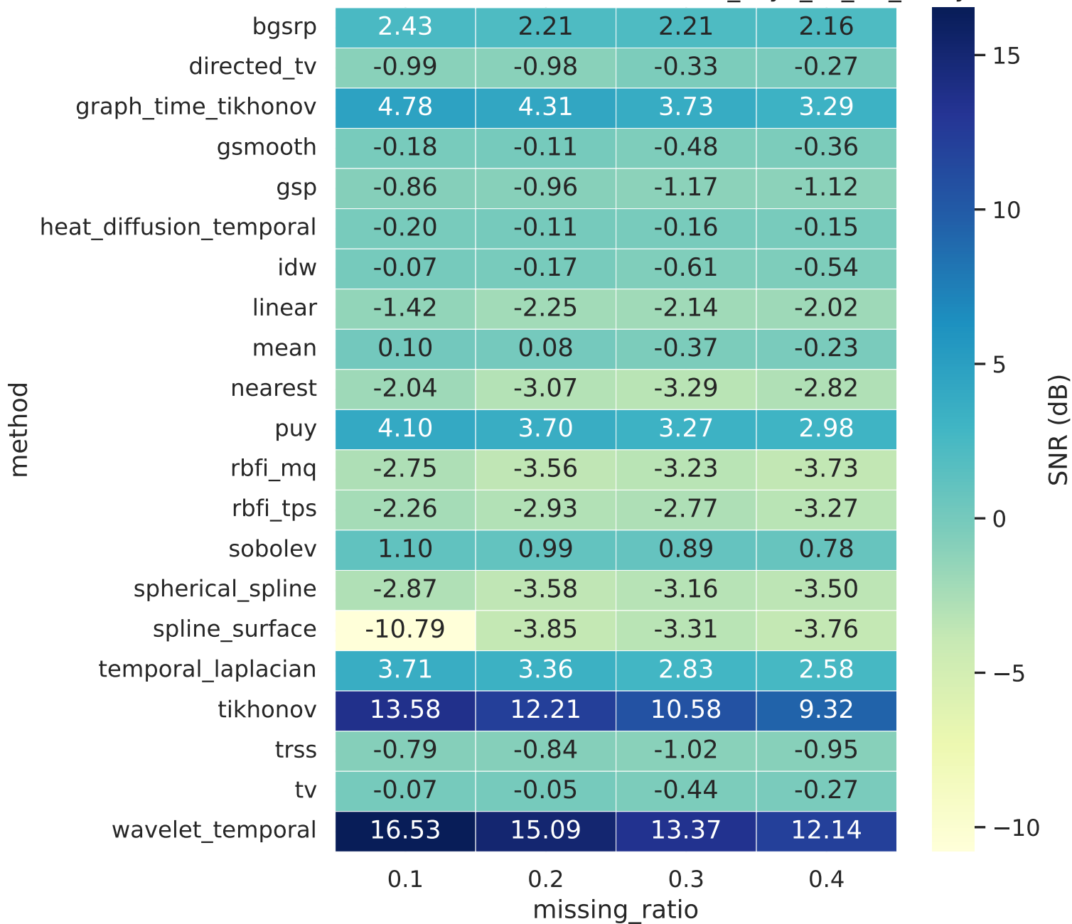
Mean SNR — Method × Scenario — it40_3syn_all_mr_analysis
