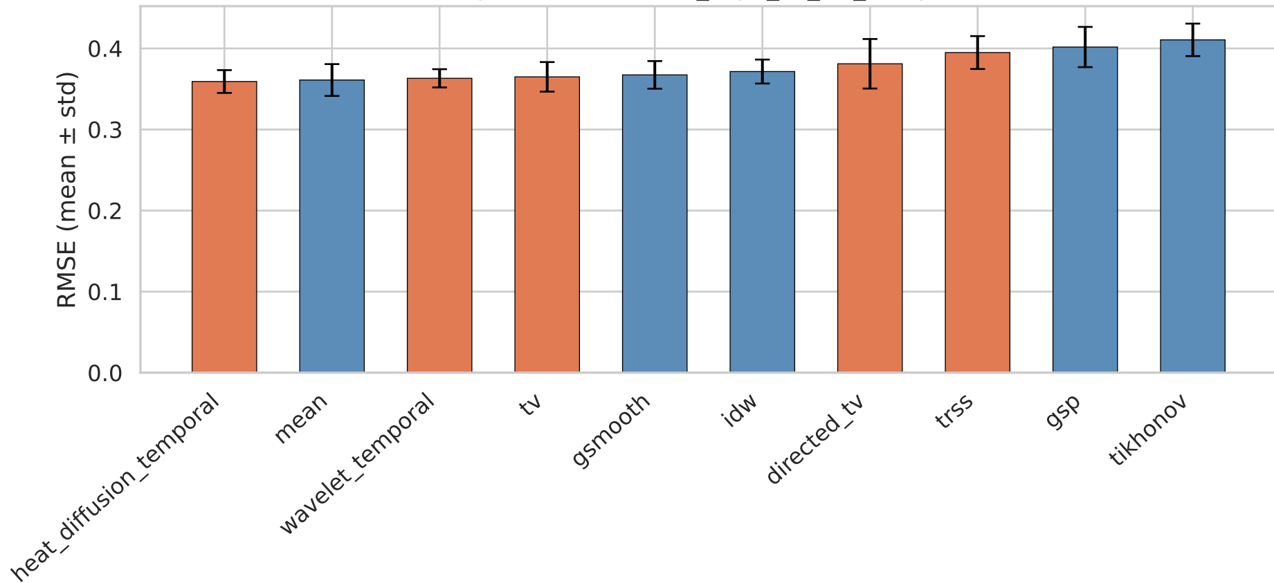
Top-10 RMSE — it40_3syn_all_mr_analysis
