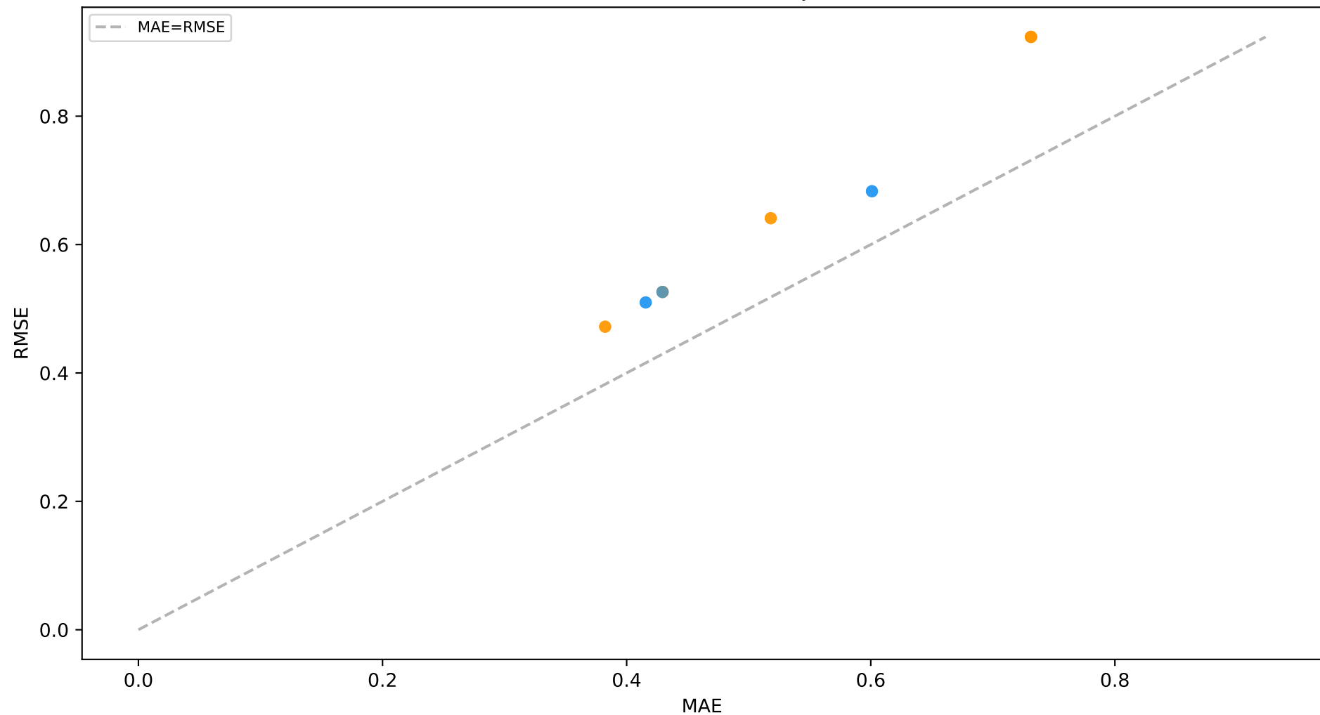
it71_few_missing_1ch_synthetic MAE vs RMSE (azul=TV, naranja=Instante)
