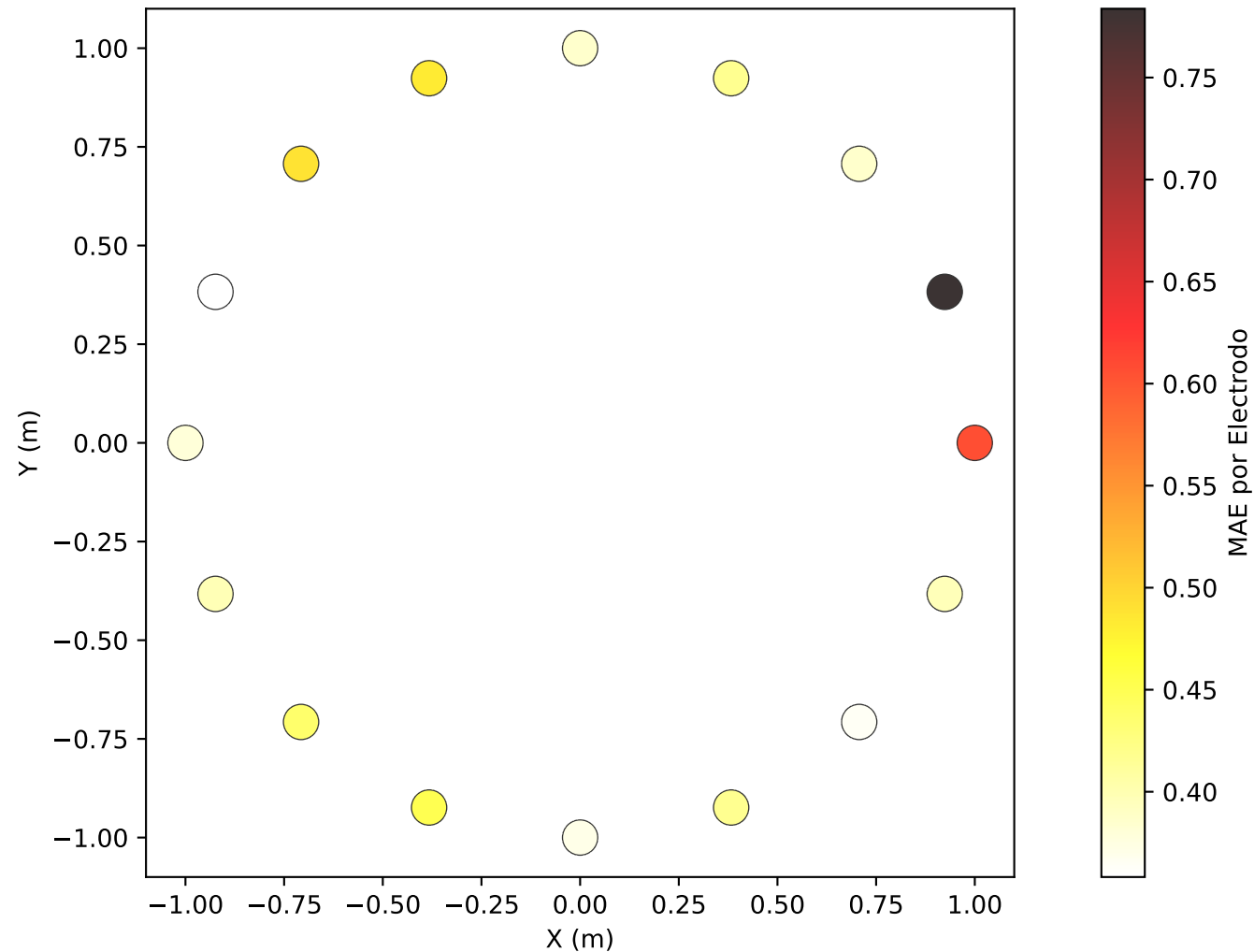
it72_few_missing_2ch_synthetic Topomap 2D: Error por Electrodo
