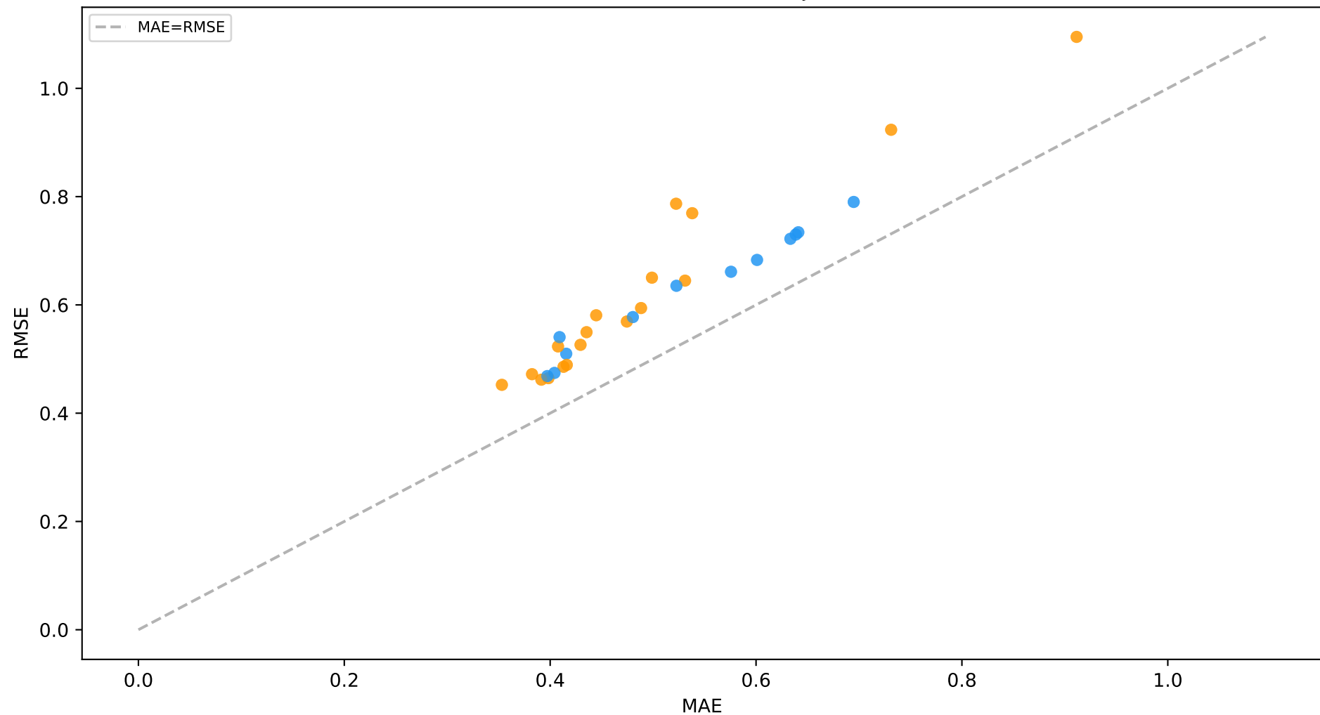
it75_few_missing_multi_synthetic MAE vs RMSE (azul=TV, naranja=Instante)
