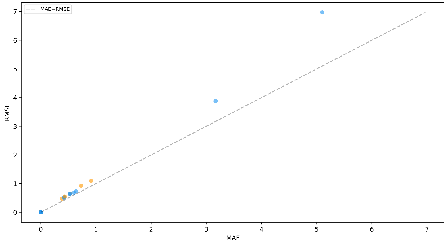
it78_few_missing_1ch_tv_focus MAE vs RMSE (azul=TV, naranja=Instante)
