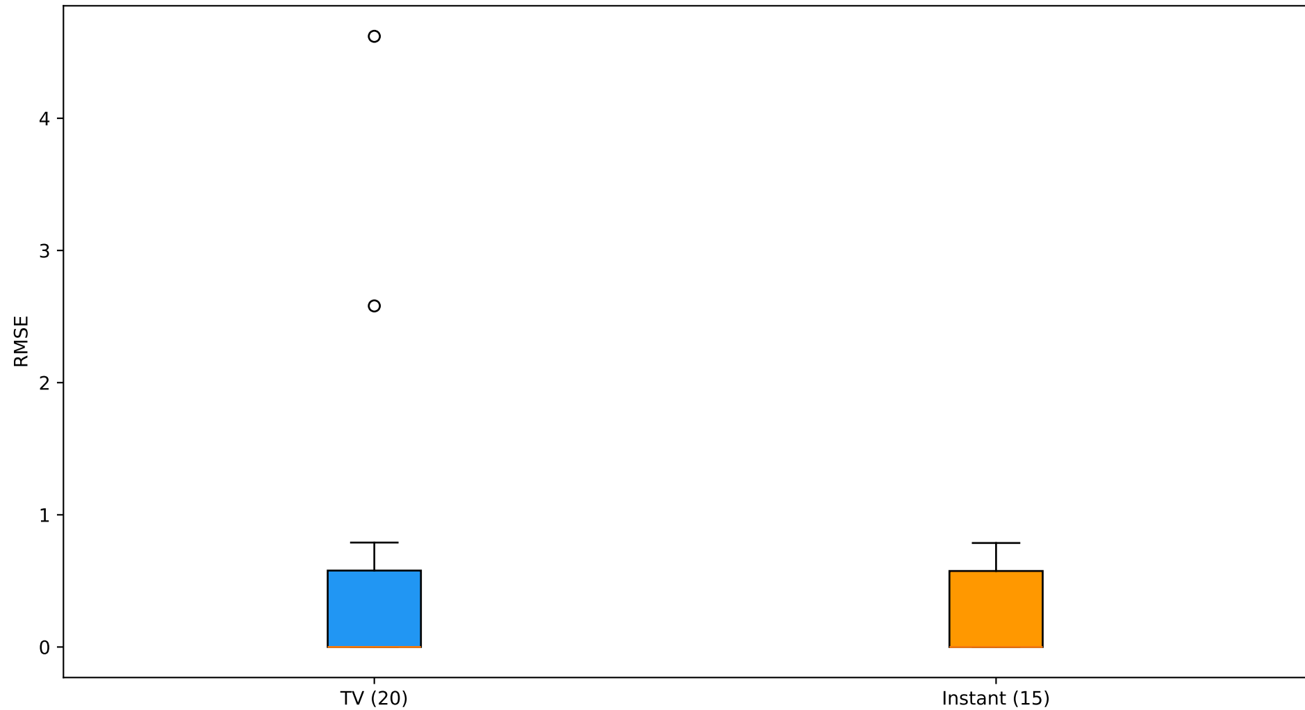
it79_few_missing_2ch_tv_focus RMSE: TV vs Métodos Instantáneos
