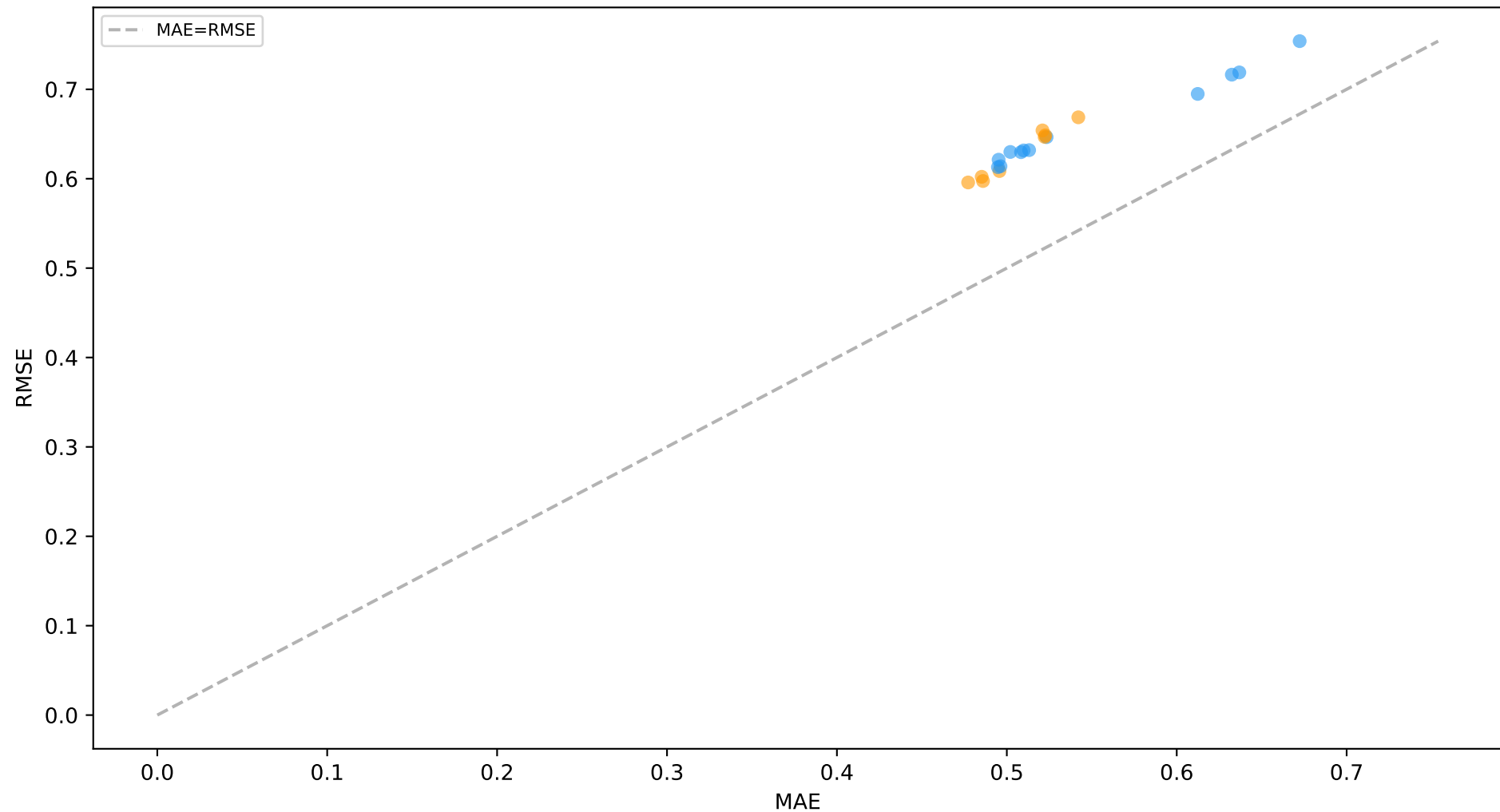
it81_instant_vs_full_synthetic MAE vs RMSE (azul=TV, naranja=Instante)
