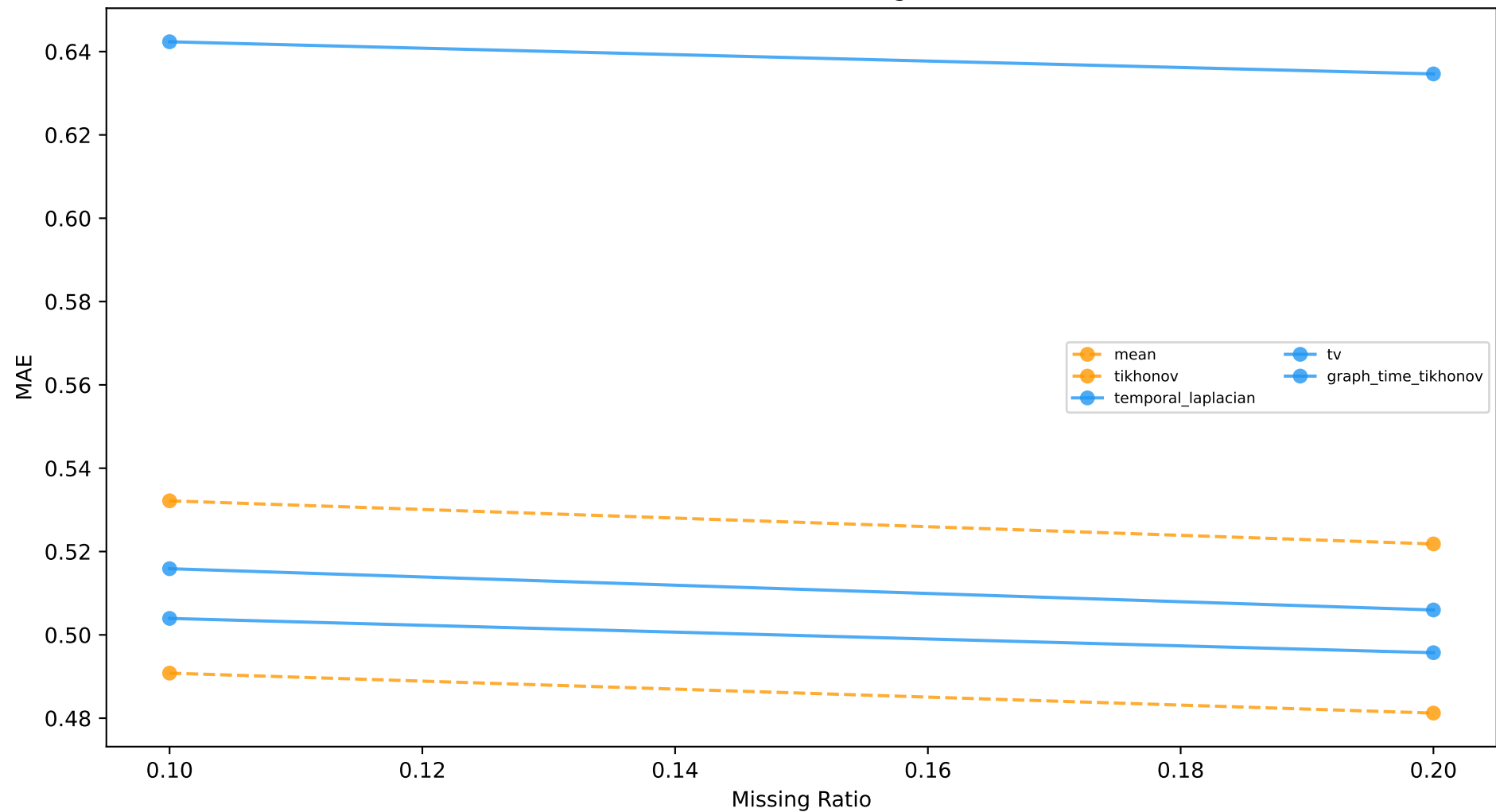
it81_instant_vs_full_synthetic Sensibilidad al Missing Ratio
