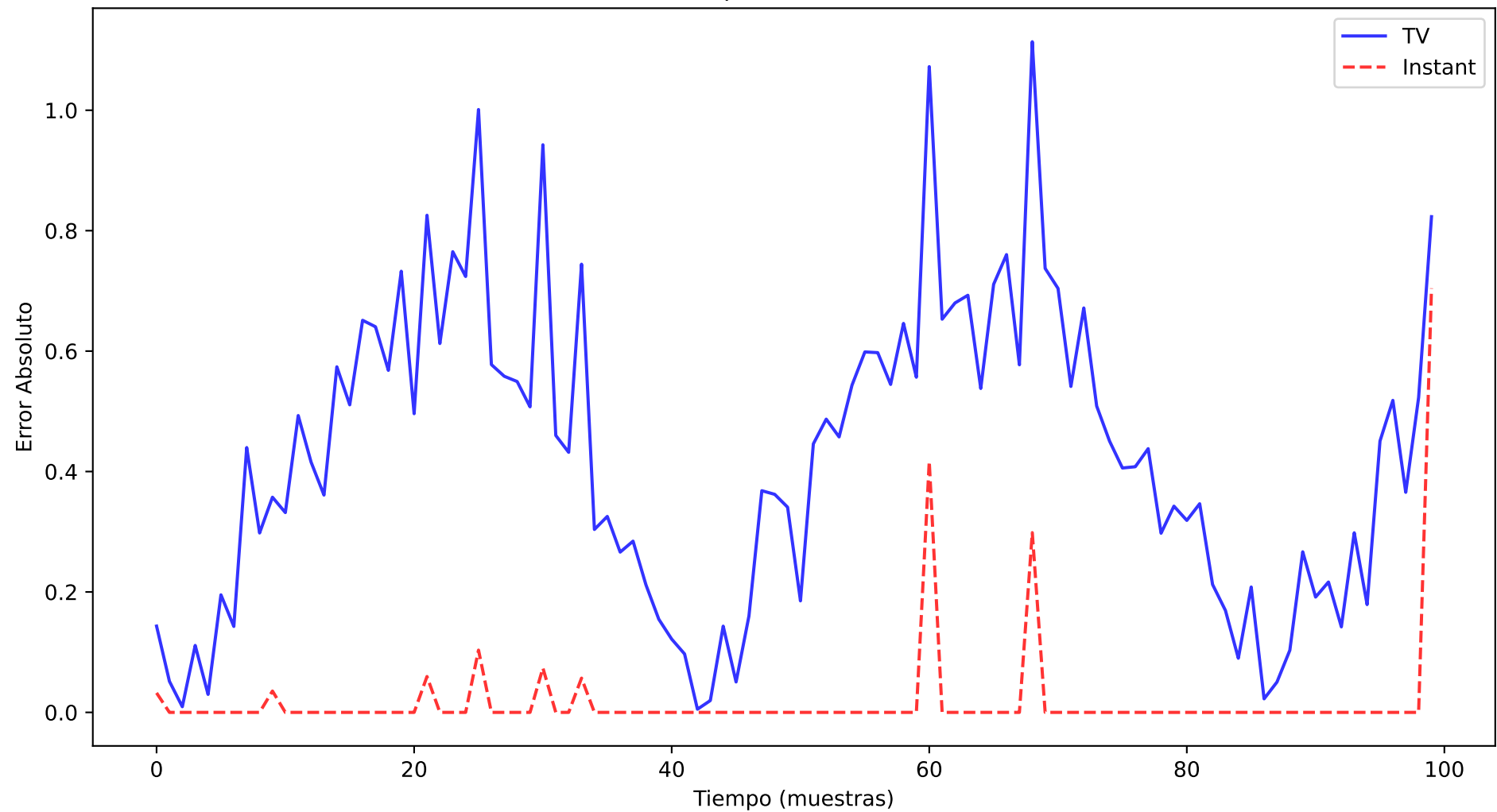
it82_full_signal_recon_synthetic Error Temporal: TV vs Instante
