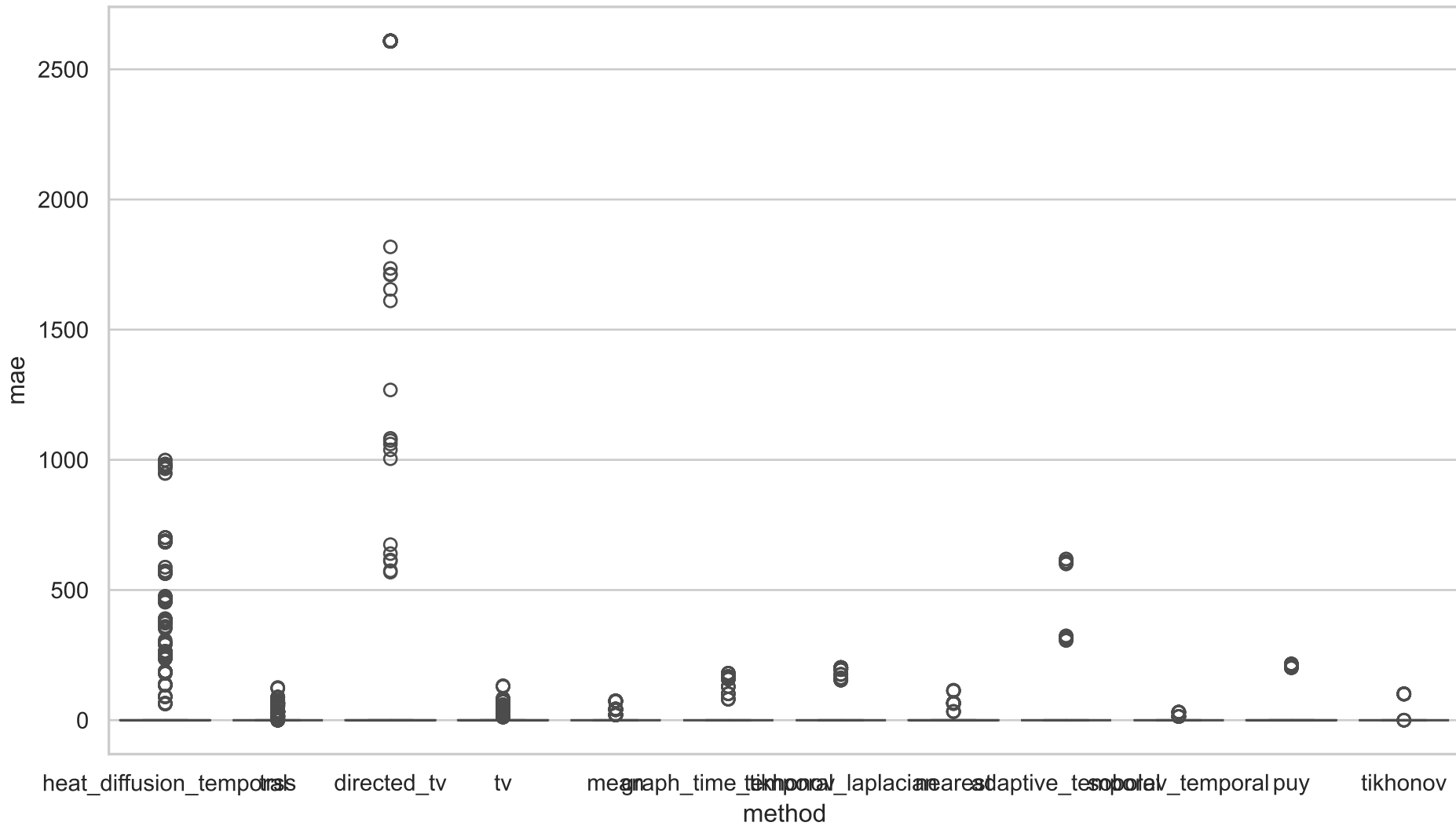
Distribution of mae by method (it131-it150)
