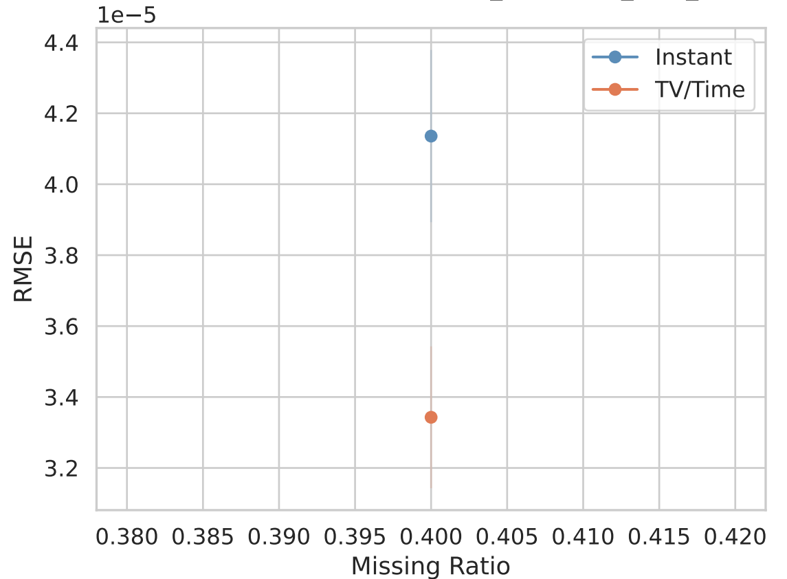
RMSE — TV/Time vs Instant — it11_physionet_high_missing
