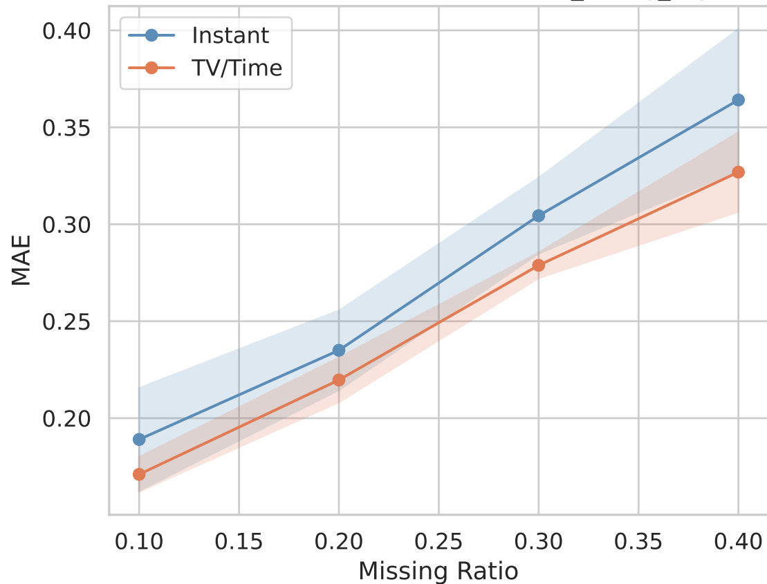
MAE — TV/Time vs Instant — it16b_vknng_3syn
