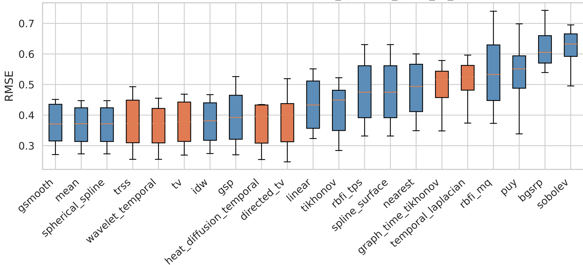
RMSE Distribution by Method — it17_synthetic_broad_all_graphs
