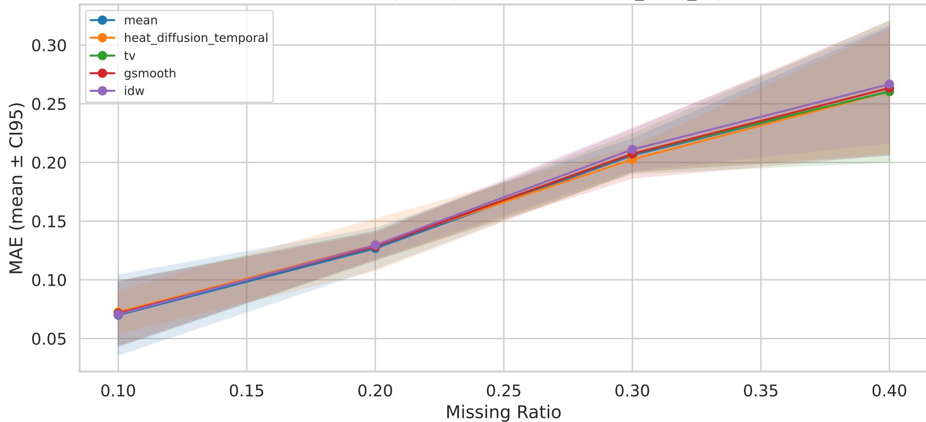
MAE Sensitivity — Top-5 Methods — it23b_knng_3syn
