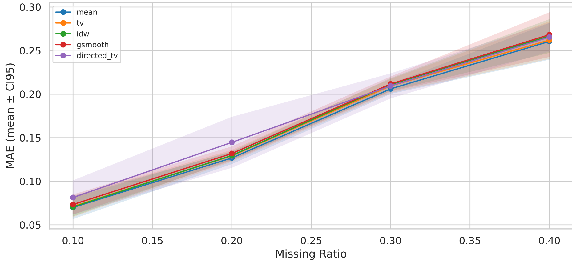
MAE Sensitivity — Top-5 Methods — it06b_kalofolias_nnk_3syn
