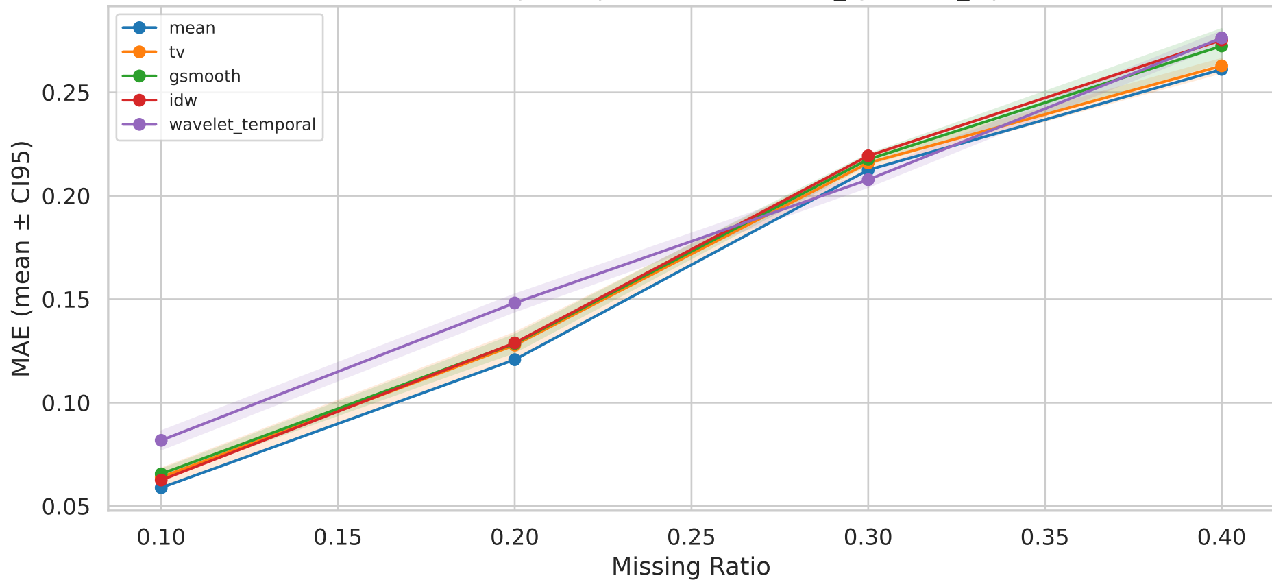
MAE Sensitivity — Top-5 Methods — it10_synthetic_alpha
