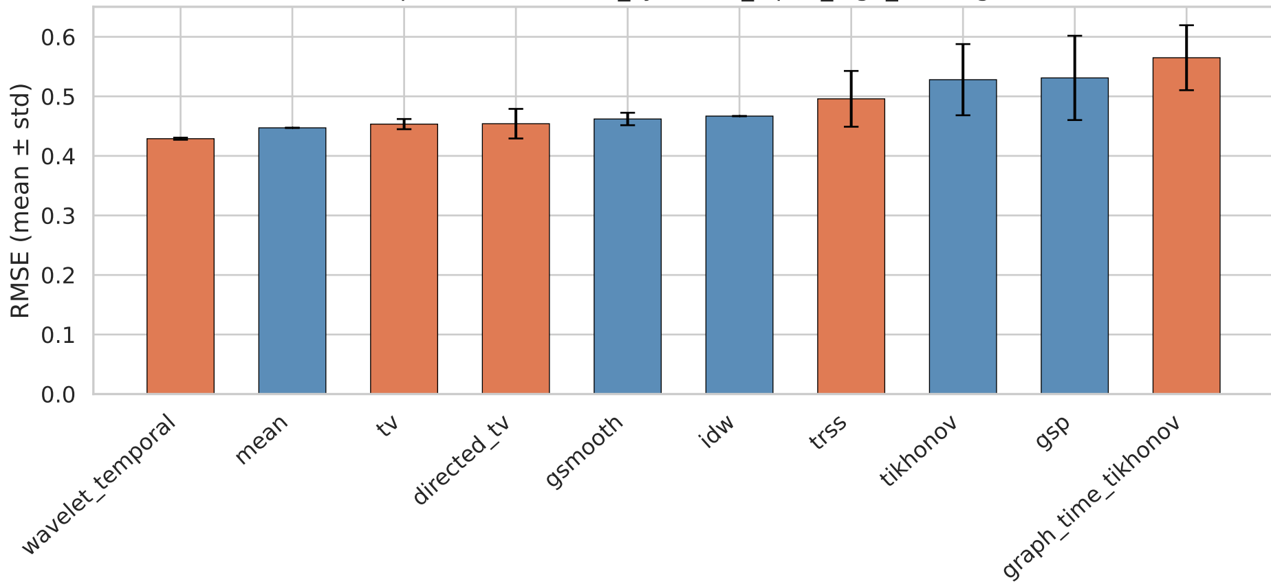
Top-10 RMSE — it20_synthetic_alpha_high_missing
