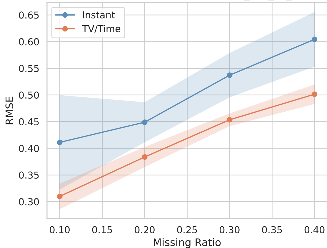
RMSE — TV/Time vs Instant — it22b_knn_k3_3syn
