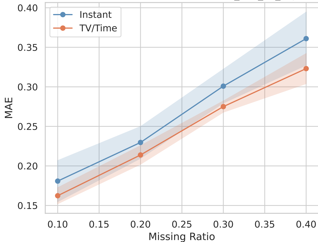
MAE — TV/Time vs Instant — it22b_knn_k3_3syn
