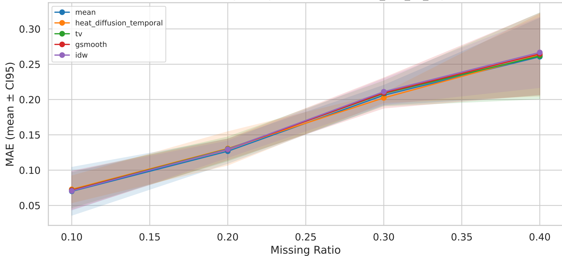
MAE Sensitivity — Top-5 Methods — it22b_knn_k3_3syn
