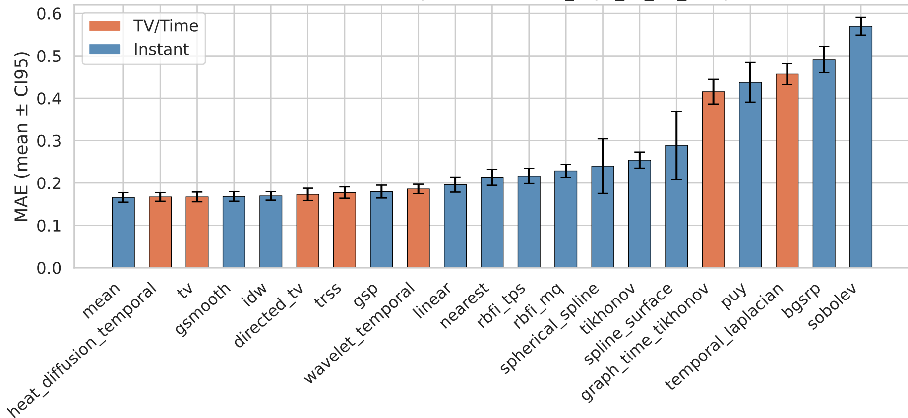
Mean Absolute Error by Method — it40_3syn_all_mr_analysis
